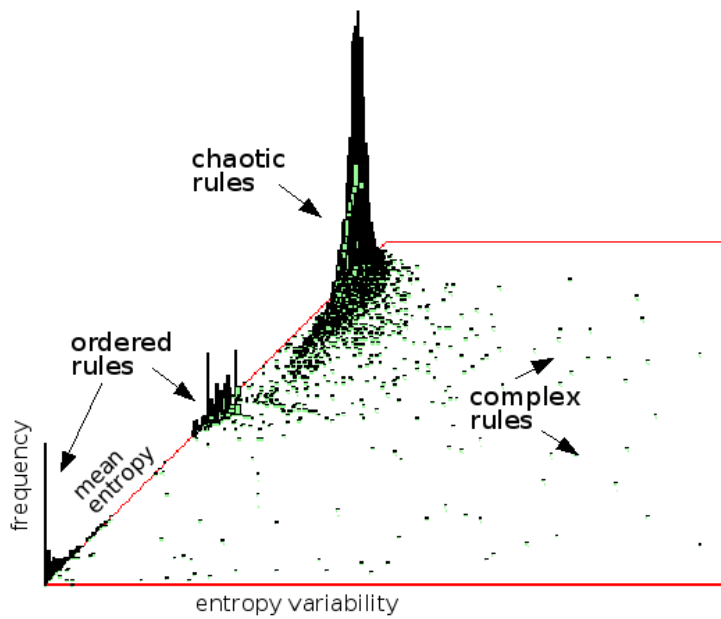
Fig. 6. Scatter plot of a sample of 15800 2d hexagonal CA rules ( v=3 , k=6 ), plotting mean entropy against entropy variability, which classifies rules between ordered, complex and chaotic. The vertical axis shows the frequency of rules at positions on the plot – most are chaotic. The plot automatically classifies rule-space.
