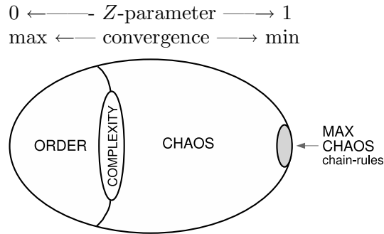
Fig. 9. A view of rule-space (after Langton[2]). Tuning the Z -parameter from 0 to 1 shifts the dynamics from maximum to minimum convergence, from order to chaos, traversing a phase transition where complexity lurks. The chain-rules on the right are maximally chaotic and have the very least convergence, decreasing with system size, making them suitable for dynamical encryption.
