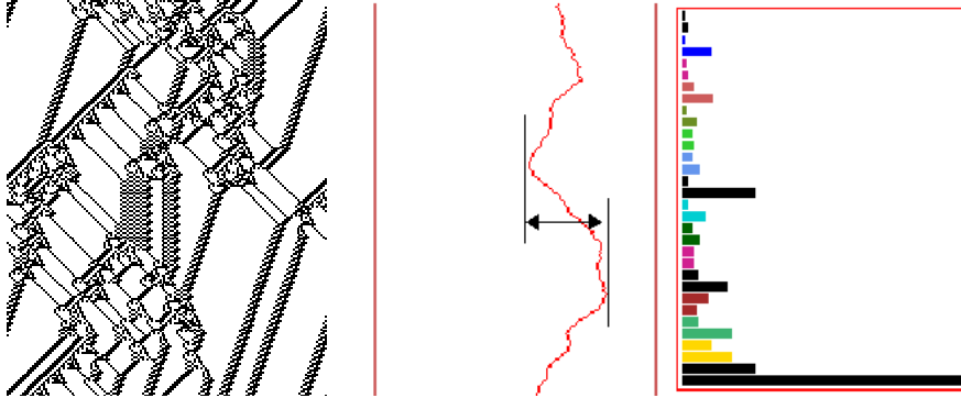
Fig. 5. Left: The space-time patterns of a 1D complex CA, n=150 about 200 time-steps. Right: A snapshot of the input frequency histogram measured over a moving window of 10 time-steps. Centre: The changing entropy of the histogram, its variability providing a non-subjective measure to discriminate between ordered, complex and chaotic rules automatically. High variability implies complex dynamics.
