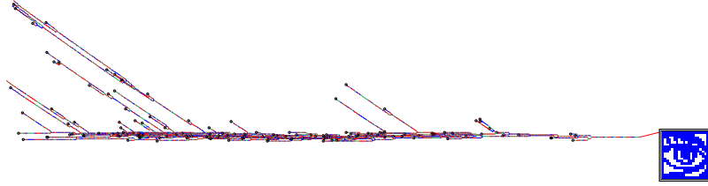
Fig. 8. A subtree of a chain-rule 1D CA n=400 . The root state (the eye) is shown in 2d ( 20 \times 20 ). Backwards iteration was stopped after 500 reverse time-steps. The subtree has 4270 states. The density of both leaf states and states that branch is very low (about 0.03) - where maximum branching equals 2.
