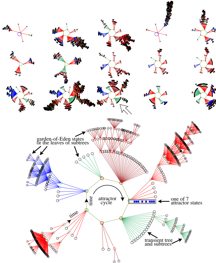
Fig. 14. Top: The basin of attraction field of a random Boolean network, k=3 , n=13 . The 2^{13} = 8192 states in state-space are organised into 15 basins, with attractor periods ranging between 1 and 7, and basin volume between 68 and 2724. Bottom: A basin of attraction (arrows above) which links 604 states, of which 523 are leaf states. The attractor period = 7, and one of the attractor states is shown in detail as a bit pattern. The direction of time is inwards, then clock-wise at the attractor.
