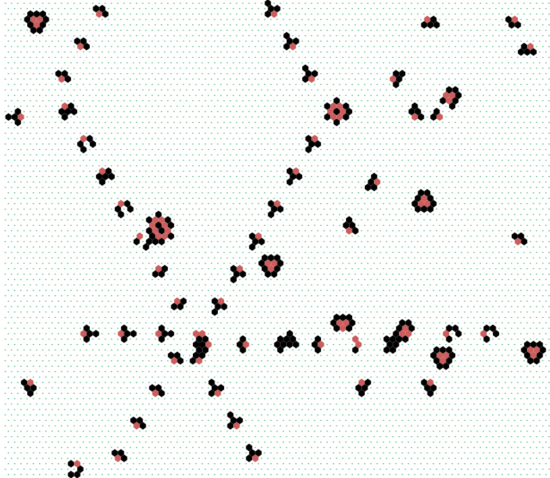
Fig. 7. A snapshot of the 3-value 2D CA spiral-rule[16] on a hexagonal lattice. n=88\times 88 , k=7 , where a diversity of interacting mobile and static structures emerge: spiral glider-guns, mobile glider-guns, self-reproduction by glider collisions. A glider moves in the direction of its red nose.
