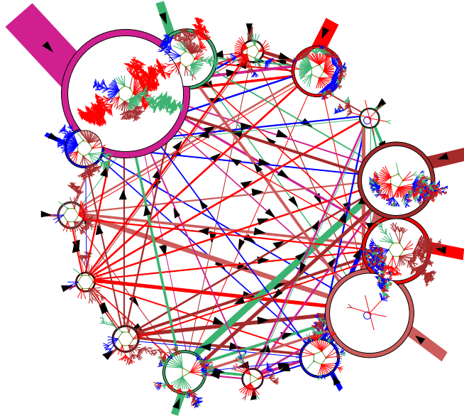
Fig. 15. The jump-graph (of the same RBN as in Fig. 14) shows the probability of jumping between basins due to single bit-flips to attractor states. Nodes representing basins are scaled according to the number of states in the basin (basin volume). Links are scaled according to both basin volume and the jump probability. Arrows indicate the direction of jumps. Short stubs are self-jumps; more jumps return to their parent basin than expected by chance, indicating a degree of stability. The relevant basin of attraction is drawn inside inside each node.
