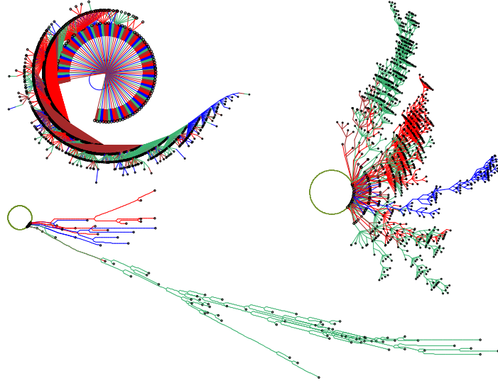
Fig. 3. Three basins of attraction with contrasting topology, n=15 , k=3 , rules 250, 110 and 30. The time flows inward towards the attractor, then clockwise. One complete set of equivalent trees is shown in each case, and just the nodes of unreachable leaf states. The topology varies from very bushy to sparsely branching, with measures such as leaf density, transient length, and in-degree distribution predicted by the rule's Z -parameter.
