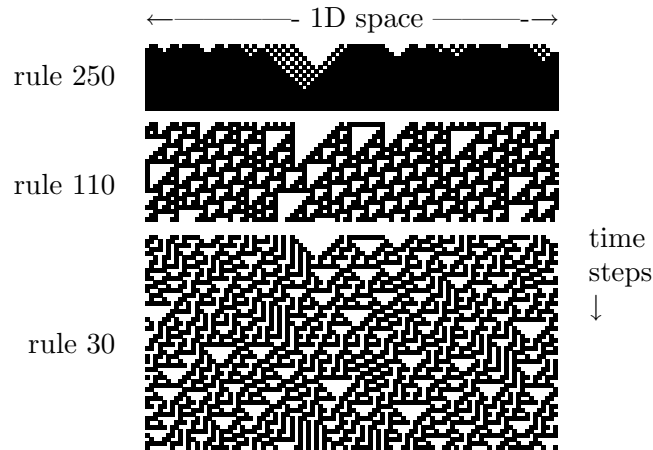
Fig. 4. 1D space-time patterns of the k=3 rules in fig.3, characteristic of order, complexity and chaos. System size n=100 with periodic boundaries. The same random initial state was used in each case. A space-time pattern is just one path through a basin of attraction.
