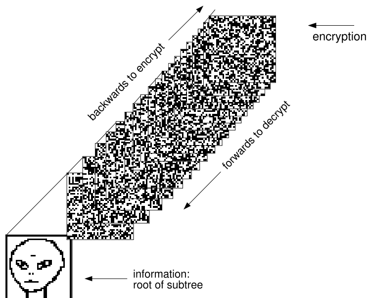
Fig. 11. A subtree of a k=7 1D CA chain-rule encrypting the “alien” root, a 1d bit-pattern displayed in 2d ( n=1600 , 40\times 40 ), but which could be ASCII, or any other form of information. Backwards iteration was stopped after 19 time-steps.
