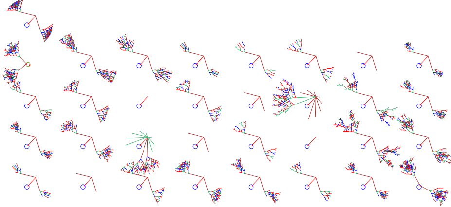
Fig. 13. Mutant basins of attraction of the v=2 , k=3 , rule 60 ( n=8 , seed all 0s). Top left: The original rule, where all states fall into just one very regular basin. The rule was first transformed to its equivalent k=5 rule (f00ff00f in hex), with 32 bits in its rule table. All 32 one-bit mutant basins are shown. If the rule is the genotype, the basin of attraction can be seen as the phenotype
